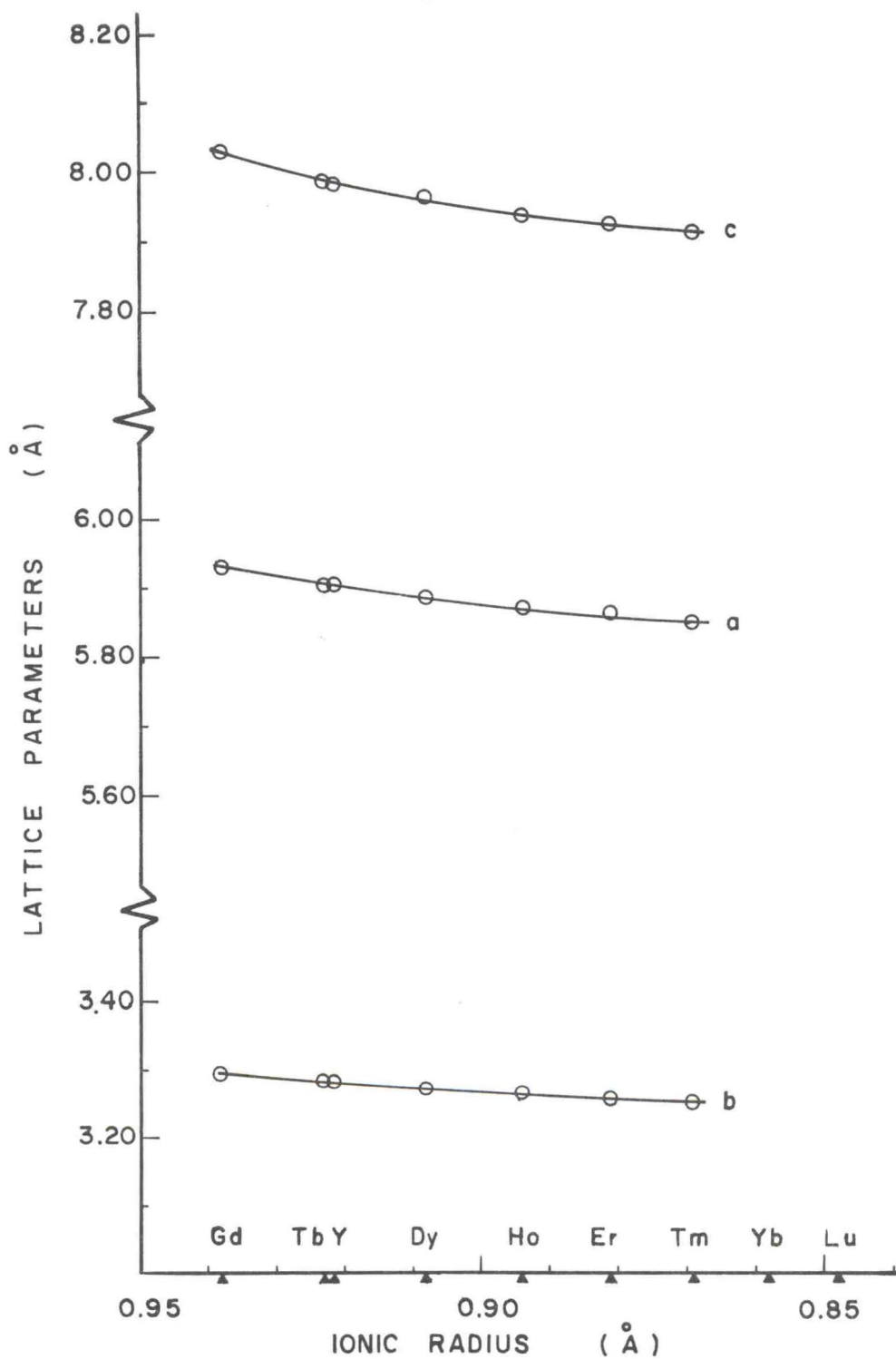
Fig. 21.--Variation of Lattice Parameters With Ionic Radius of High Pressure Orthorhombic Type Rare Earth Diantimonides.
